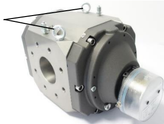
Fig. 6 | Lifting lugs
