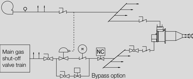
Modulating Gas with Fixed Air Control
