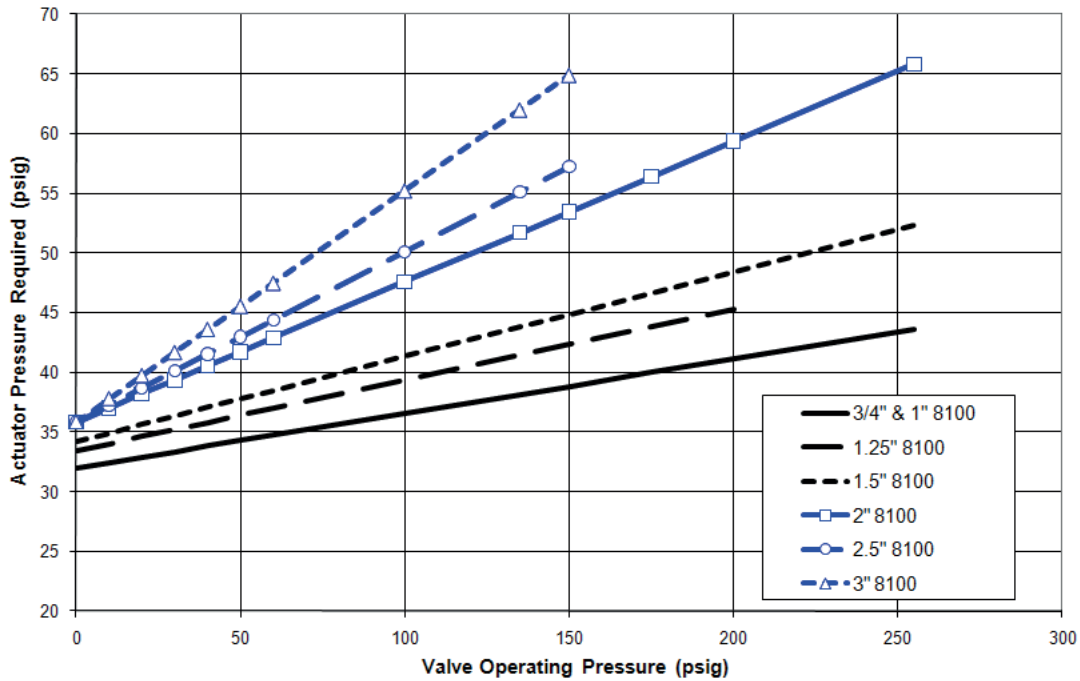
Pressure Required to Actuator Series 8100: .75"-3"
