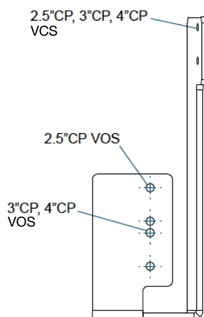
Figure 5: IP67 Switch Bracket
