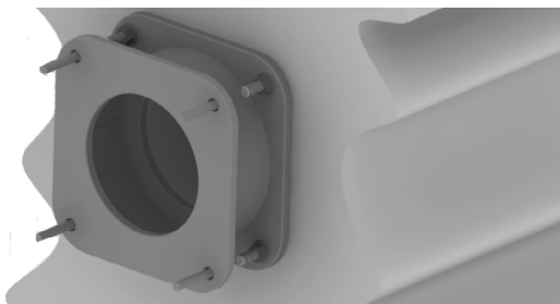
Fig. 4. Mounting Extension furnace wall
