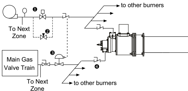
Fig. 7. High/Low Air & Gas Control
