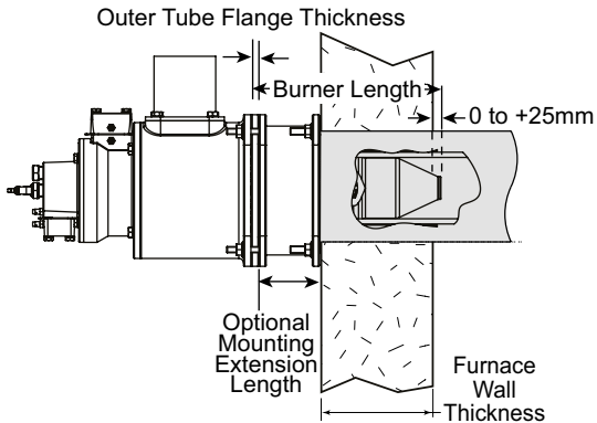
Fig. 3. Mounting Extension Length
