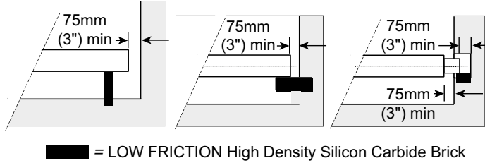
Fig. 2. Metallic Outer Tube Mounting Support
