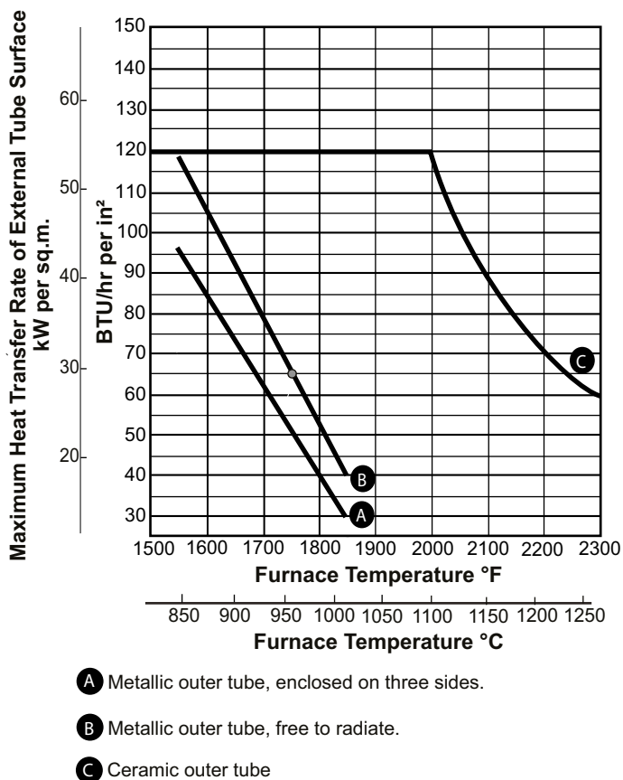
Fig. 6. Recommended Heat Flux
