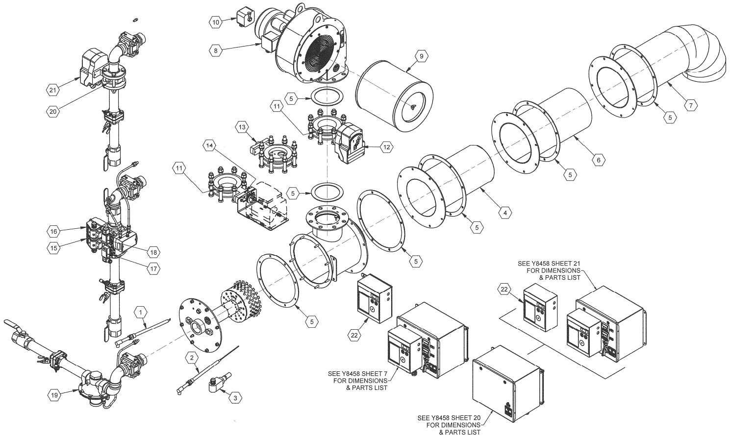
Y8458 Sht.18 (NOT TO SCALE)
