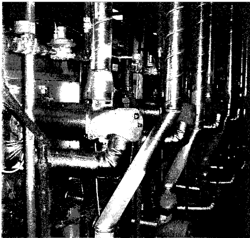
Bayonet-Ultra Recuperators provide pre-heated combustion to Eclipse TFB Burners
