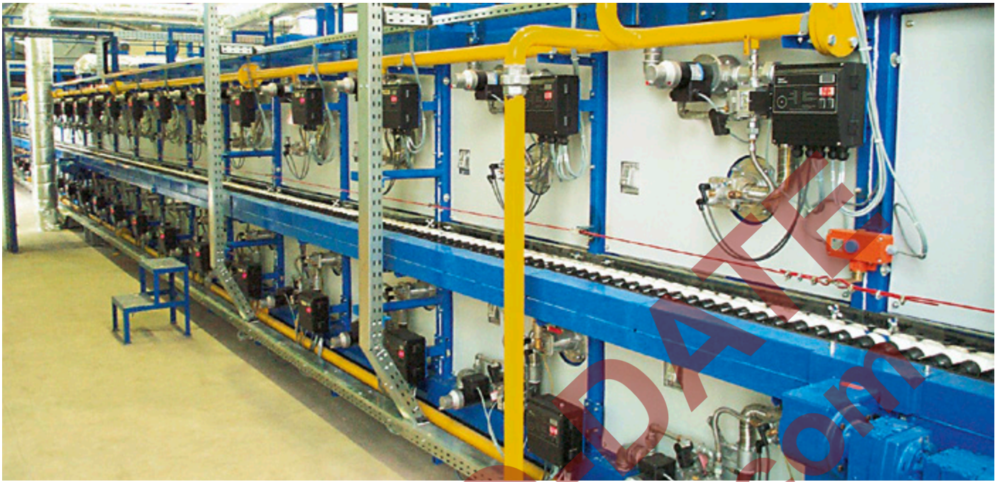
Roller hearth kiln, works photograph Laeis Bucher
